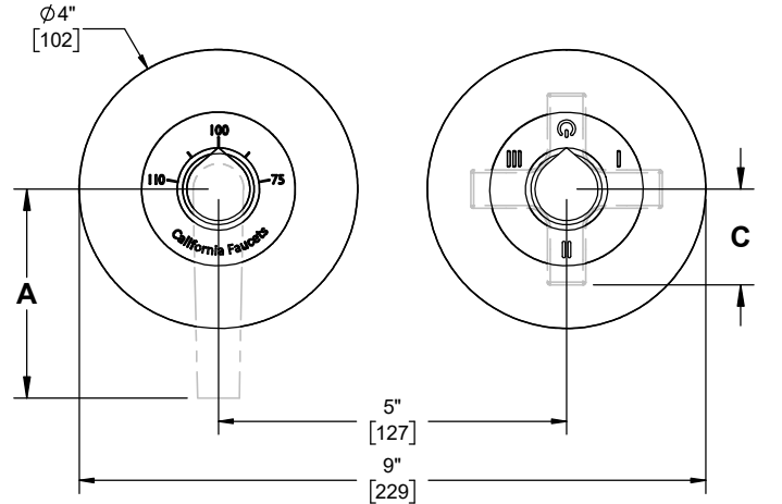
Horizontal Mounted
