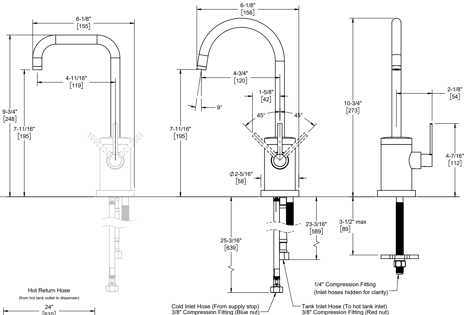
9623Q-K55-TG shown
