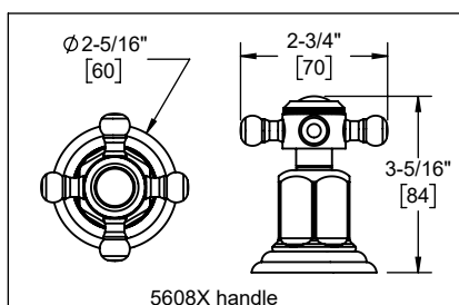
5608X handle
